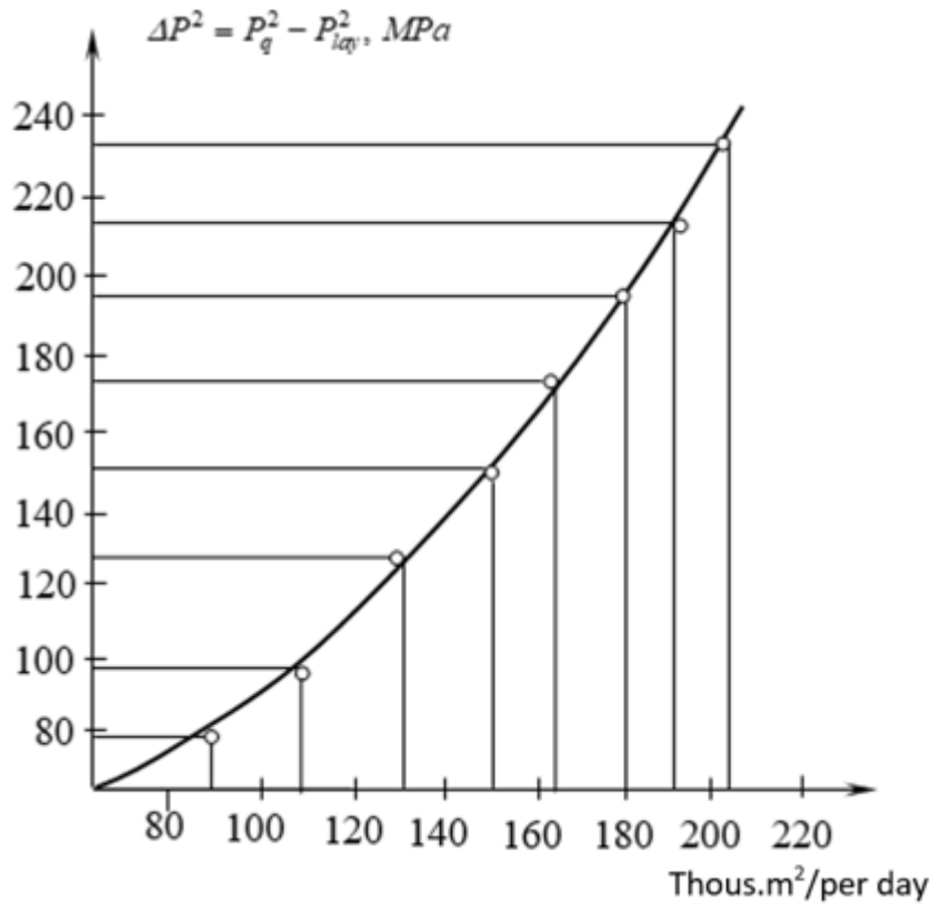
Figure 1. Underground gas storage gas well No. 415 indicator diagram
